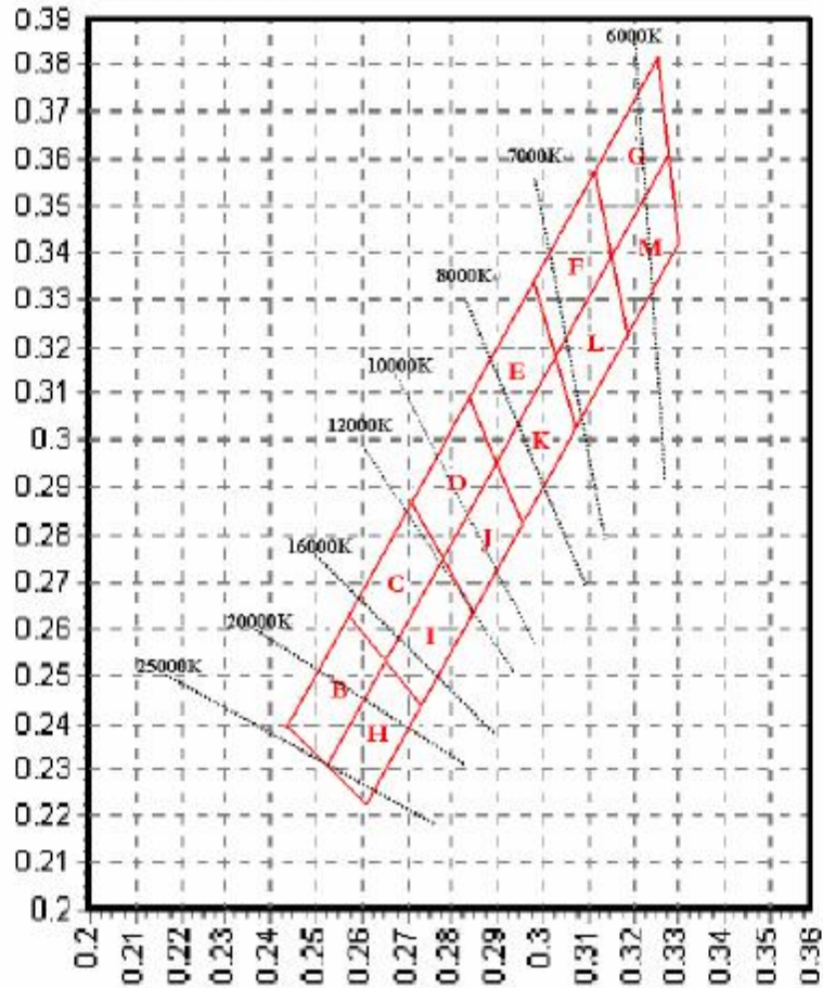
CIE 1931 Chromaticity Diagram
